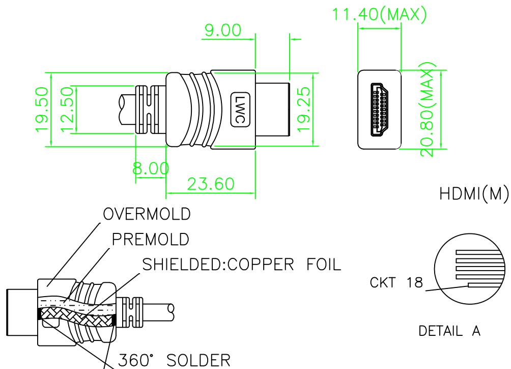
HDMI(M) SHIELDED FIG.
